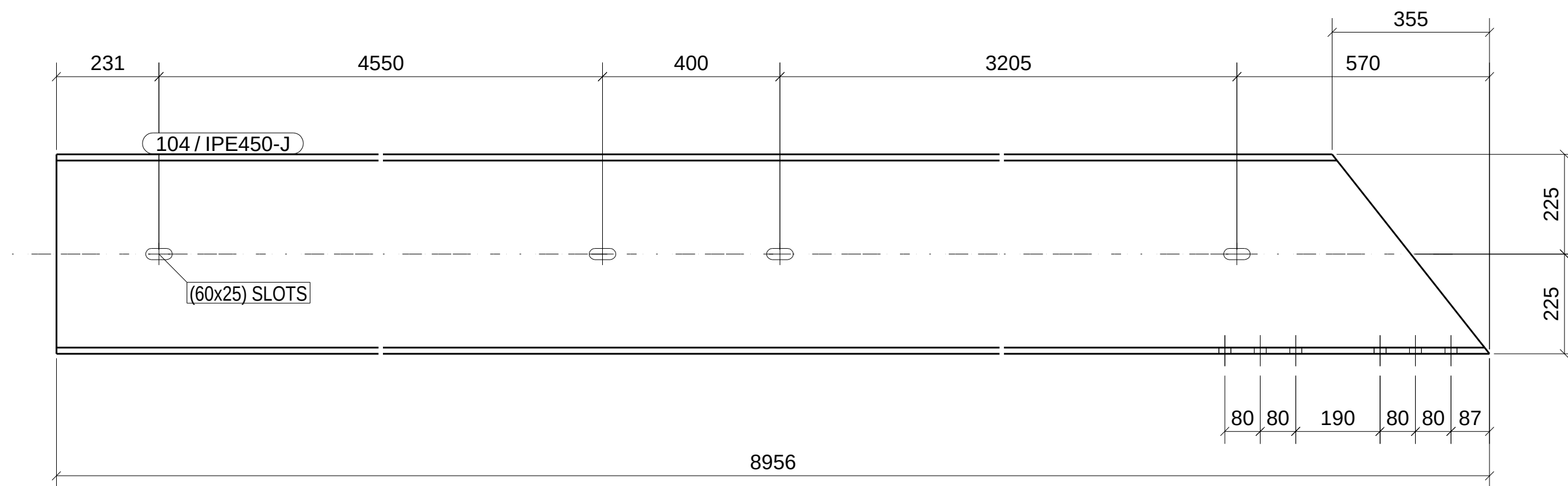
FRONT VIEW
